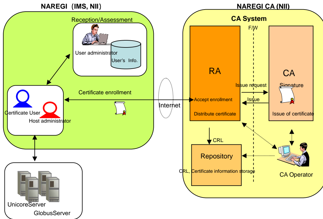
Fig.1-2 NAREGI CA System Architecture
